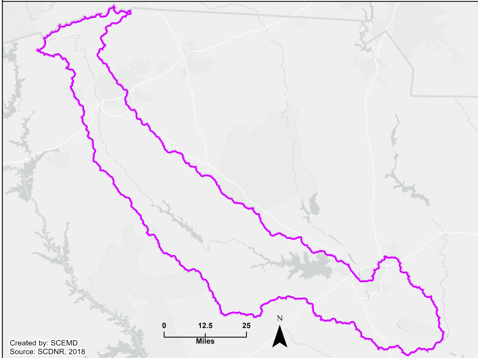
Figure 24: Saluda Watershed
