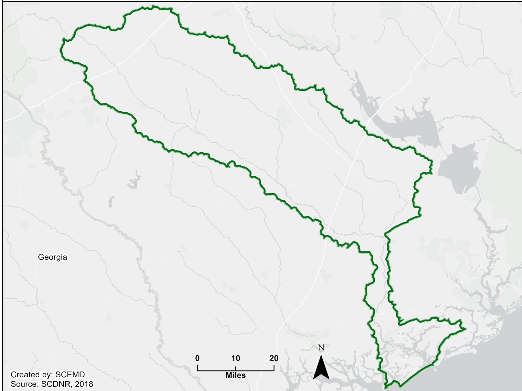
Figure 12: Edisto Watershed
