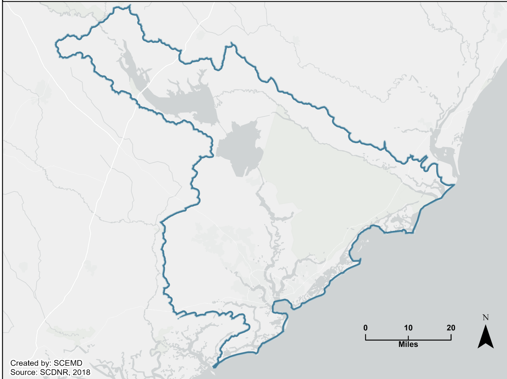
Figure 28: Santee Watershed
