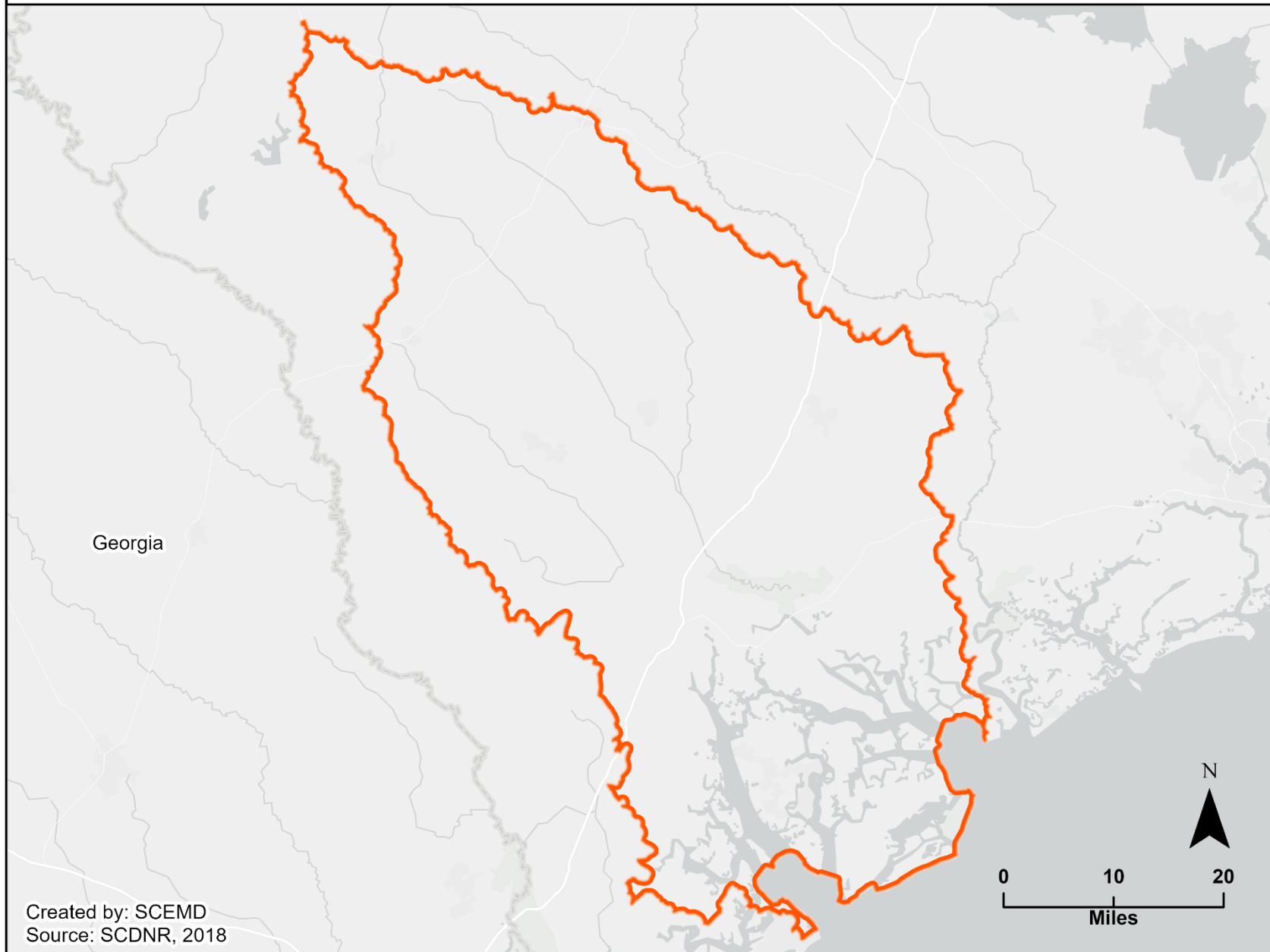
Figure 20: Salkehatchie Watershed
