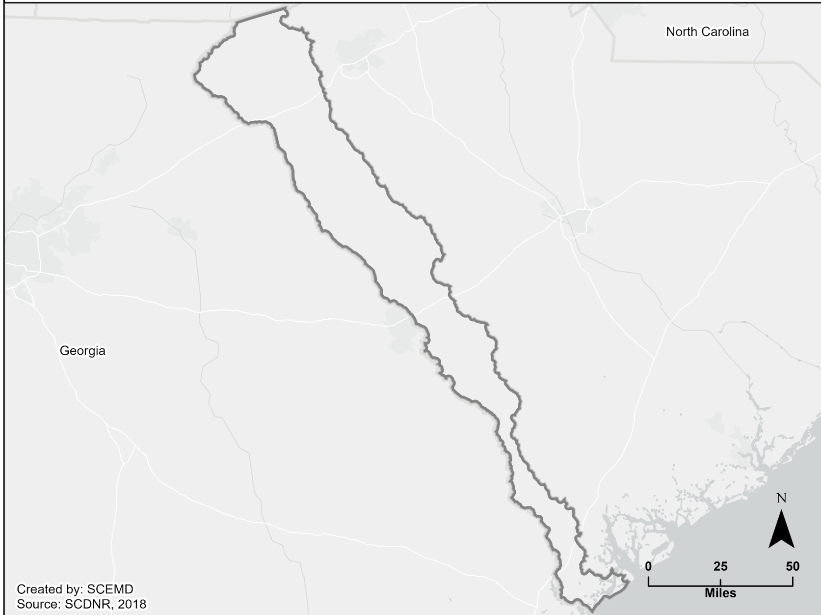
Figure 32: Savannah Watershed
