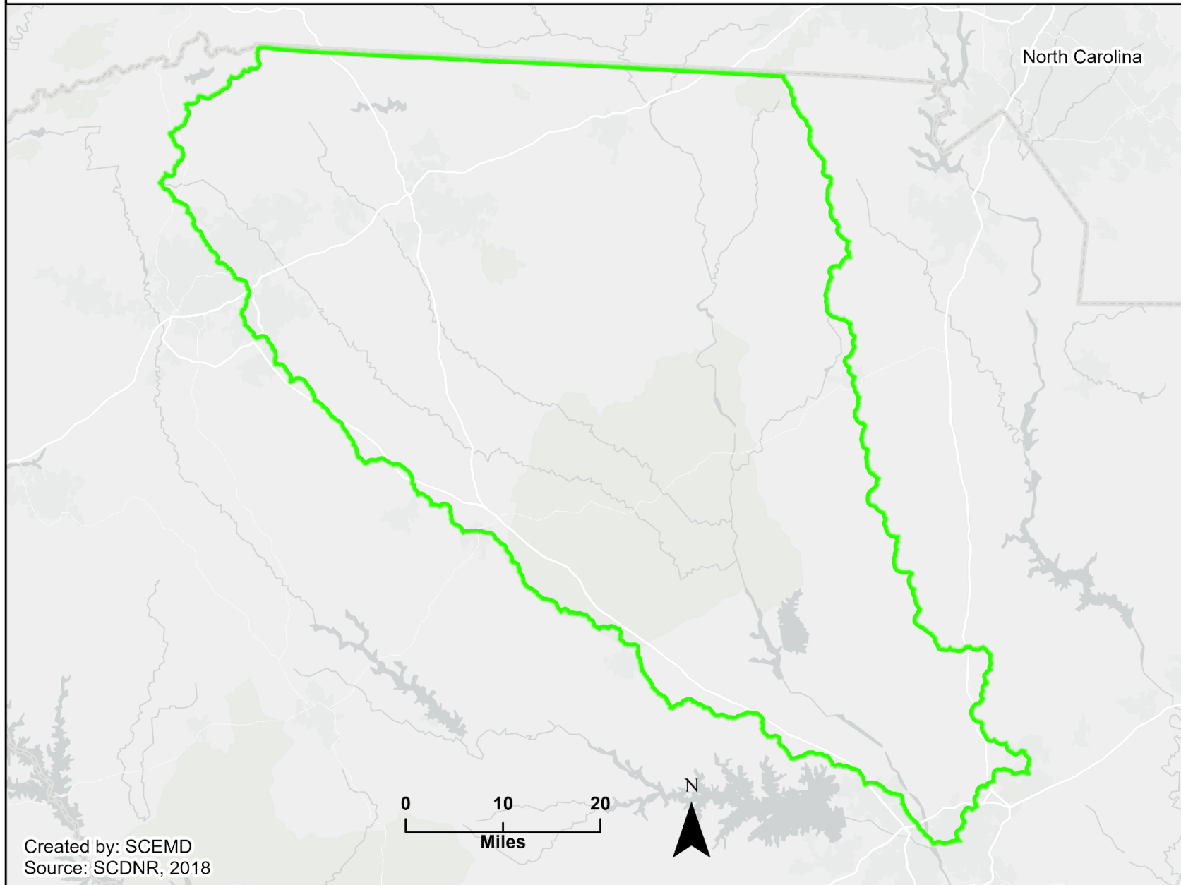
Figure 4: Broad Watershed
