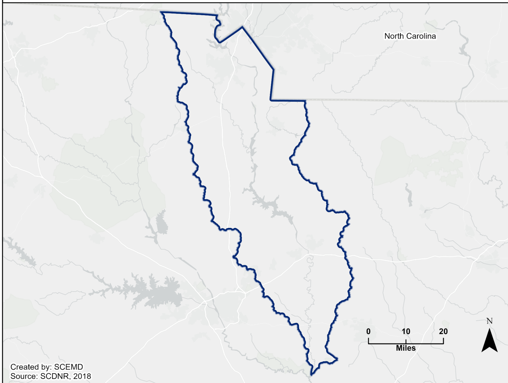
Figure 8: Catawba Watershed
